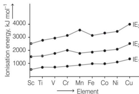
Variation of the IE_1 , IE_2 and IE_3 for the first transition metals
